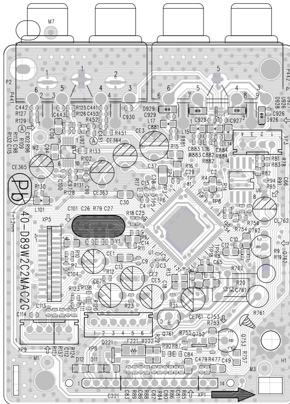
Main Board Print-layout(top side):
